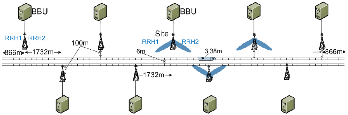
Figure 6.1.5-2: 30GHz deployment
