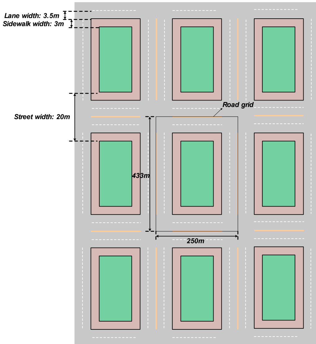
Figure 6.1.10-1: Road configuration for urban grid
